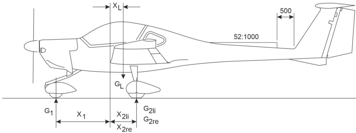
Weighing Schematic
